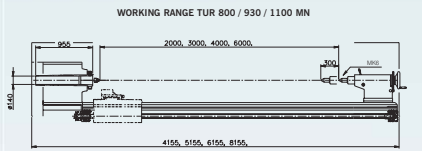
With 8-position toolturret (VDI 50)
