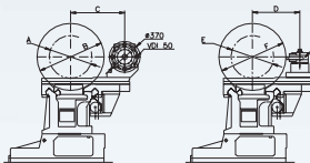
OVERALL DIMENSIONS FAT CNC TUR 800 / 930 / 1100 MN
